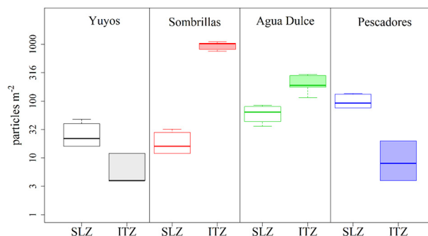
Fig. 2. Boxplot of the microplastic abundance (particles \text{m}^{-2} ) per beach and beach zone. SLZ: supralitoral zone, and ITZ: intertidal zone.
